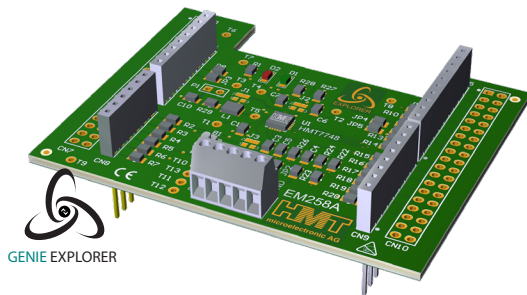
Fig.1: EM259 Development PCB
