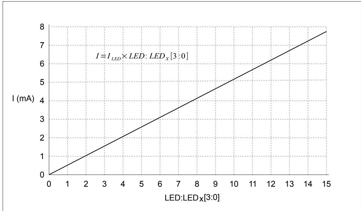
Fig. 13: HMT7748 LED currents
