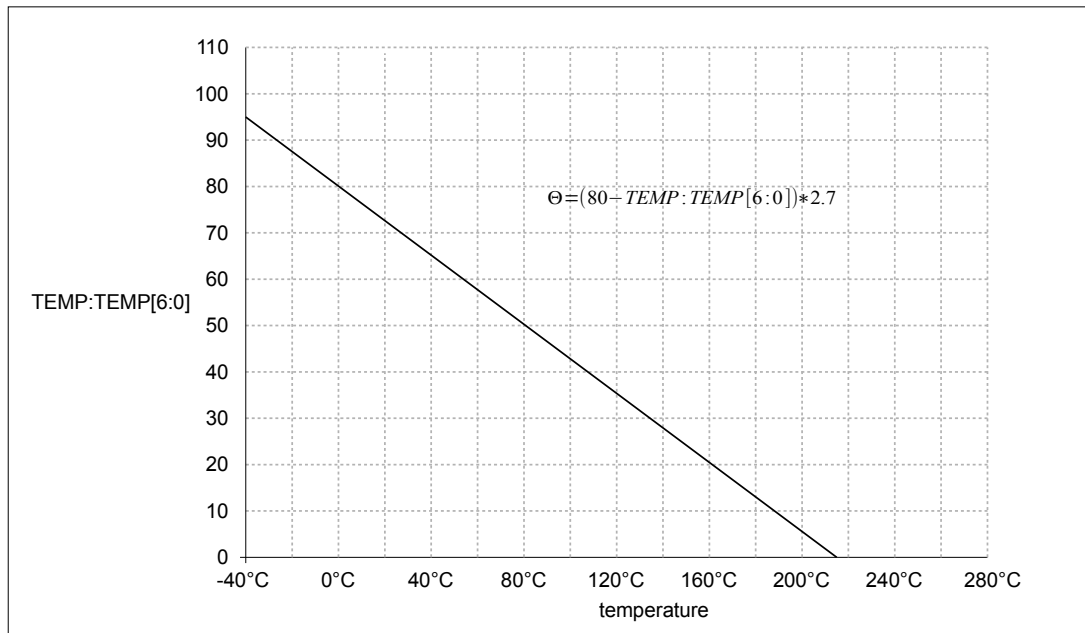
Fig. 11 HMT7748 temperature measurement
