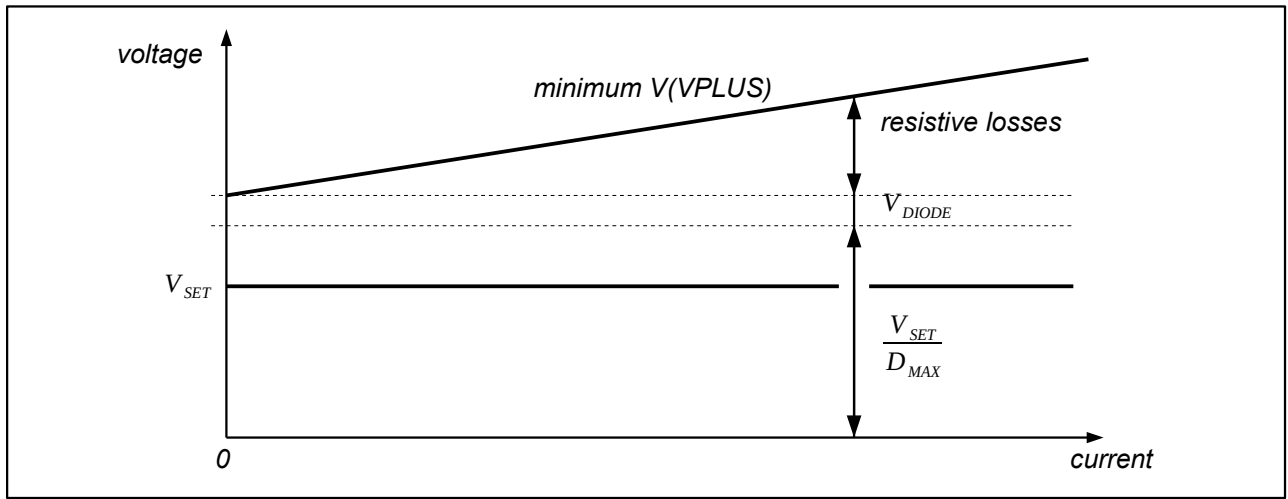
Fig. 15: Minimum supply voltage
