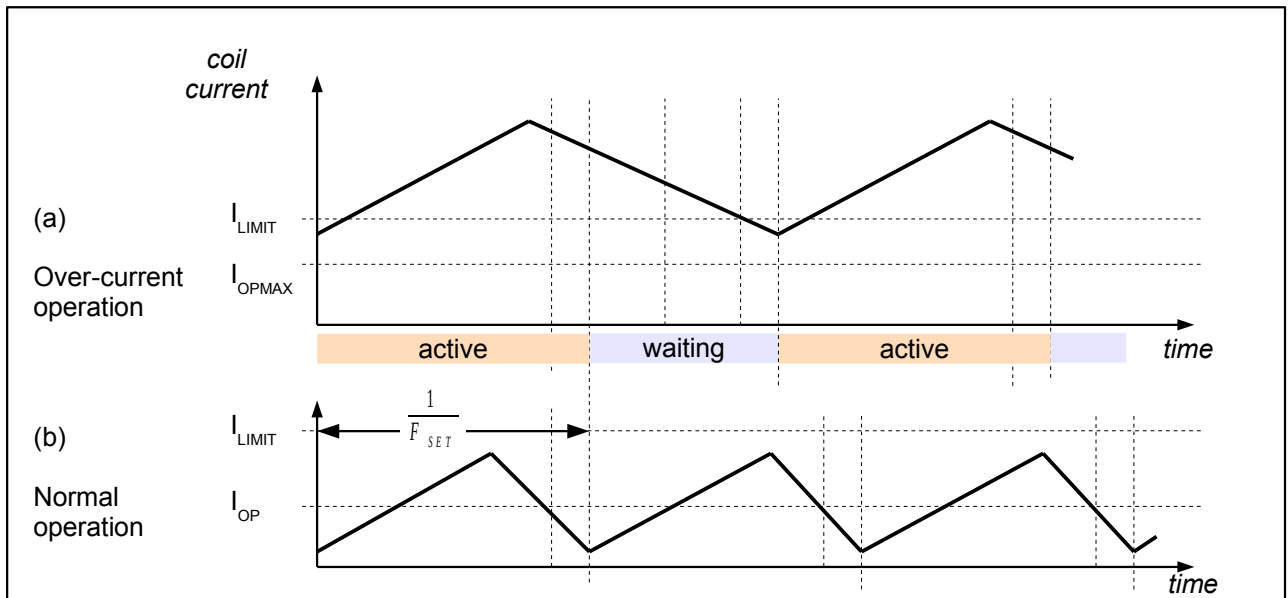
Fig. 16: Over-current operation
