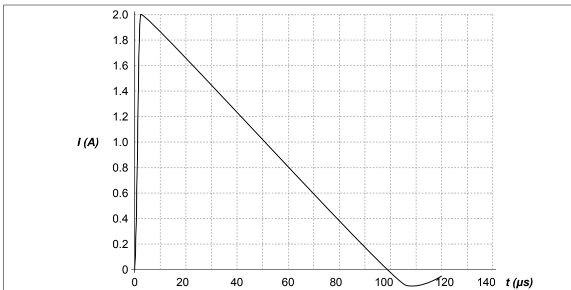
Fig. 20: Surge waveform
