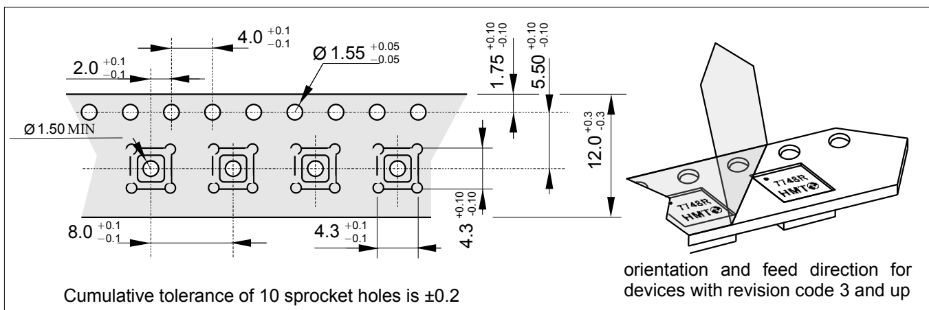
Fig. 22 Package, footprint and tape drawings for QFN
