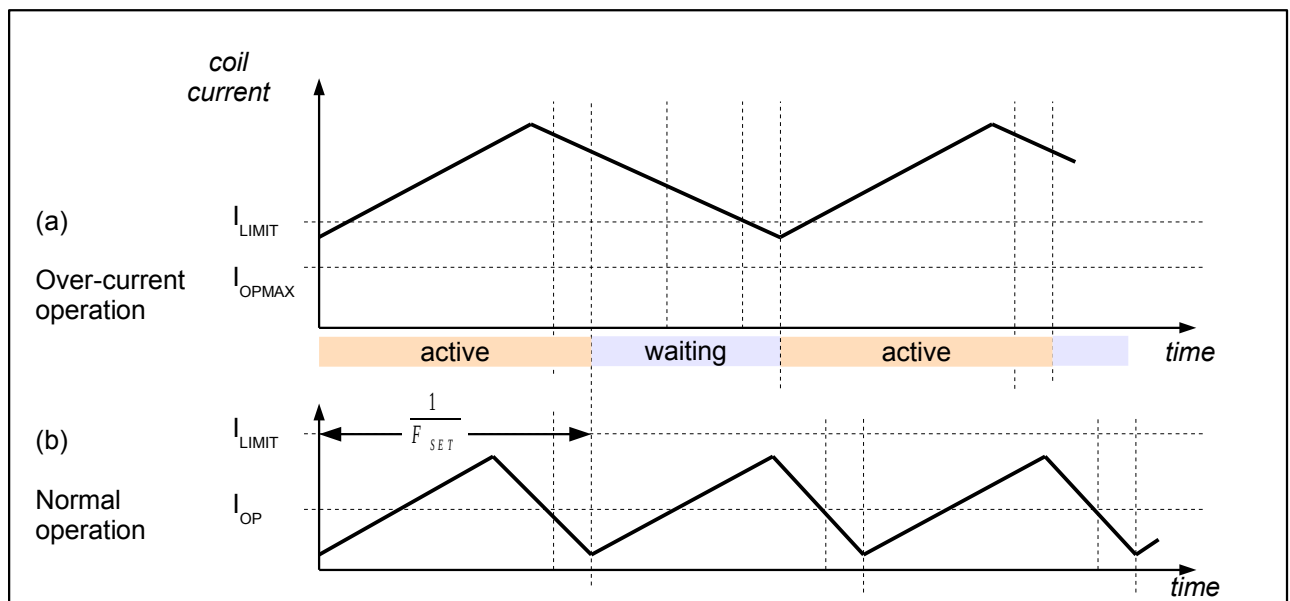
Fig. 16: Over-current operation
