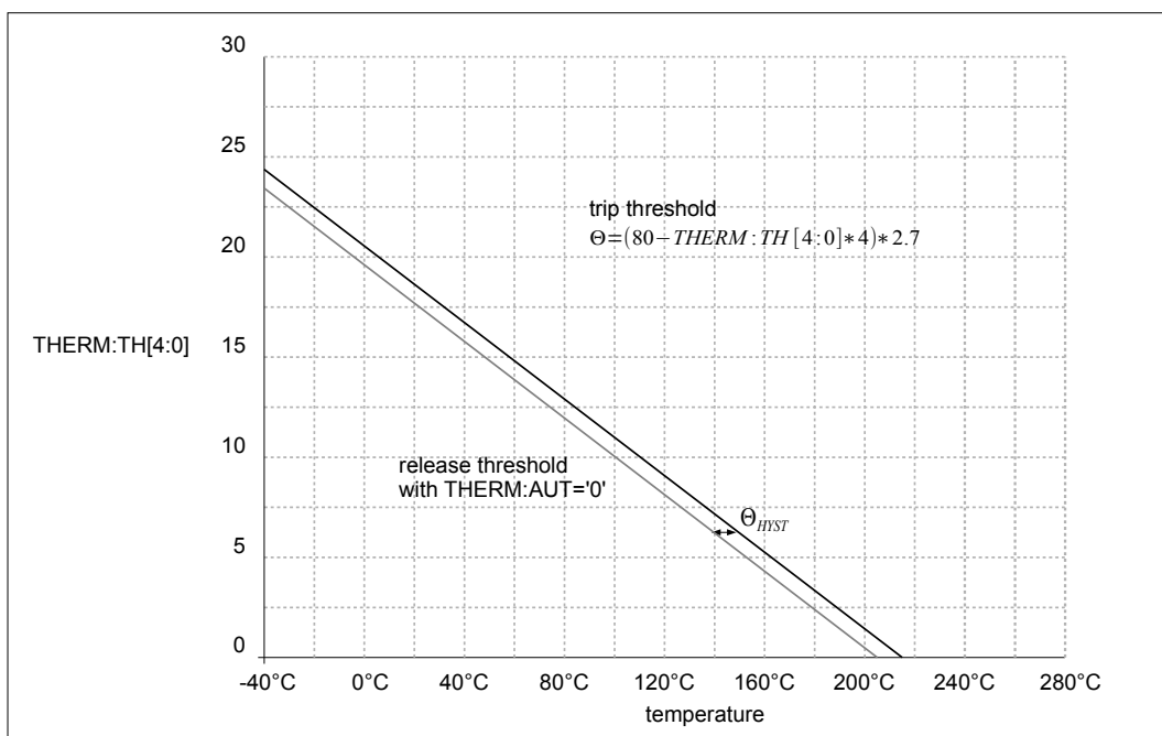
Fig. 12 HMT7748 thermal shutdown configuration
