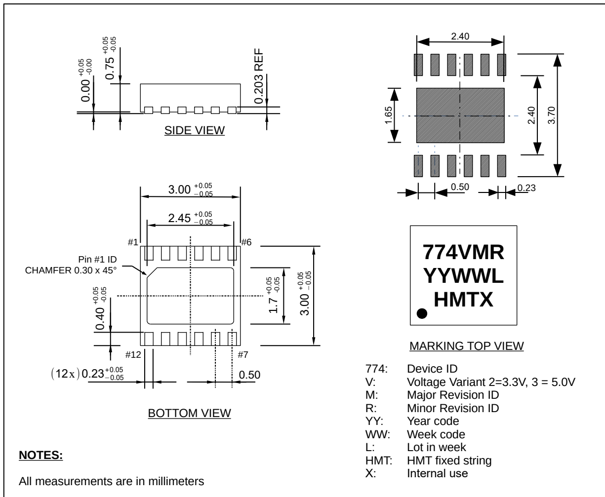
Fig. 16: Package and footprint drawing proposal for new designs
