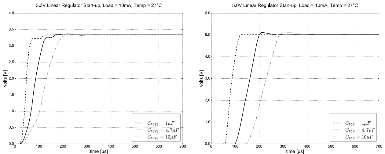
Fig. 13 Linear regulator dynamic start-up under different conditions of C_{SNS}
