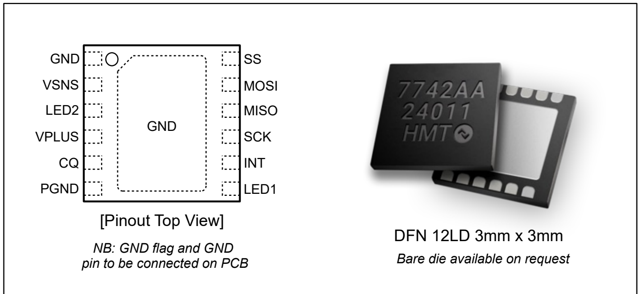
Fig. 2: Package and pinout (see §23 on page 26)
