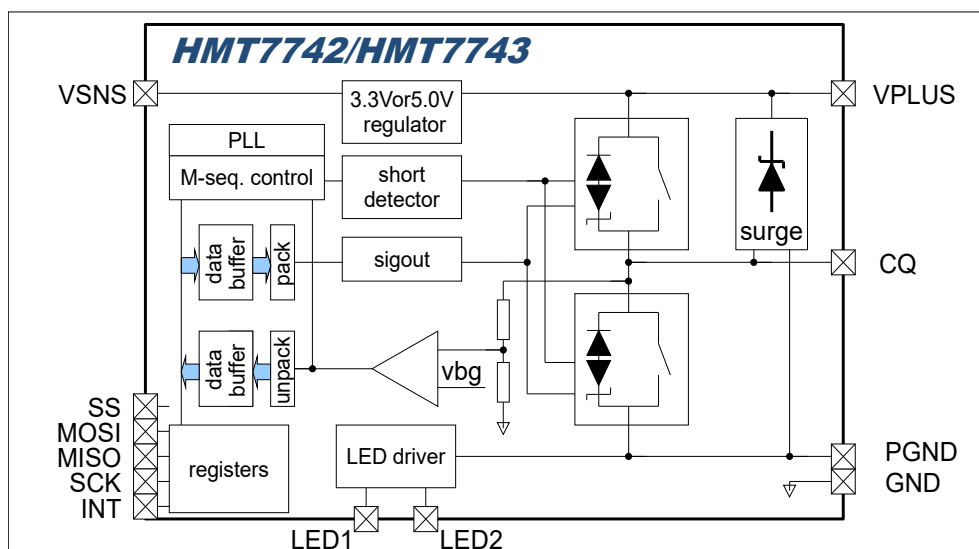
Fig. 1: Overview diagram, see Fig. 15 for a detailed block diagram
