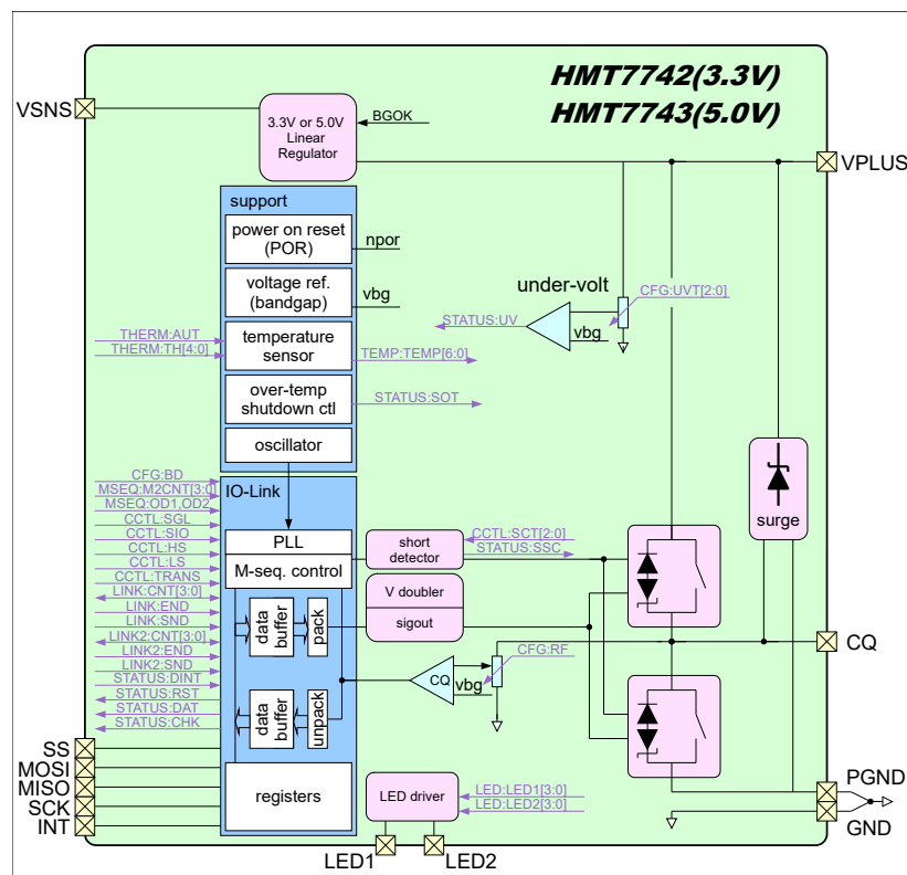
Fig. 15 Detailed block diagram, showing register field connections
