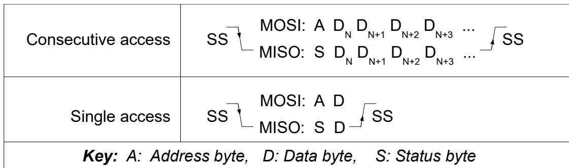
Fig. 5 Single byte and sequential byte accesses
