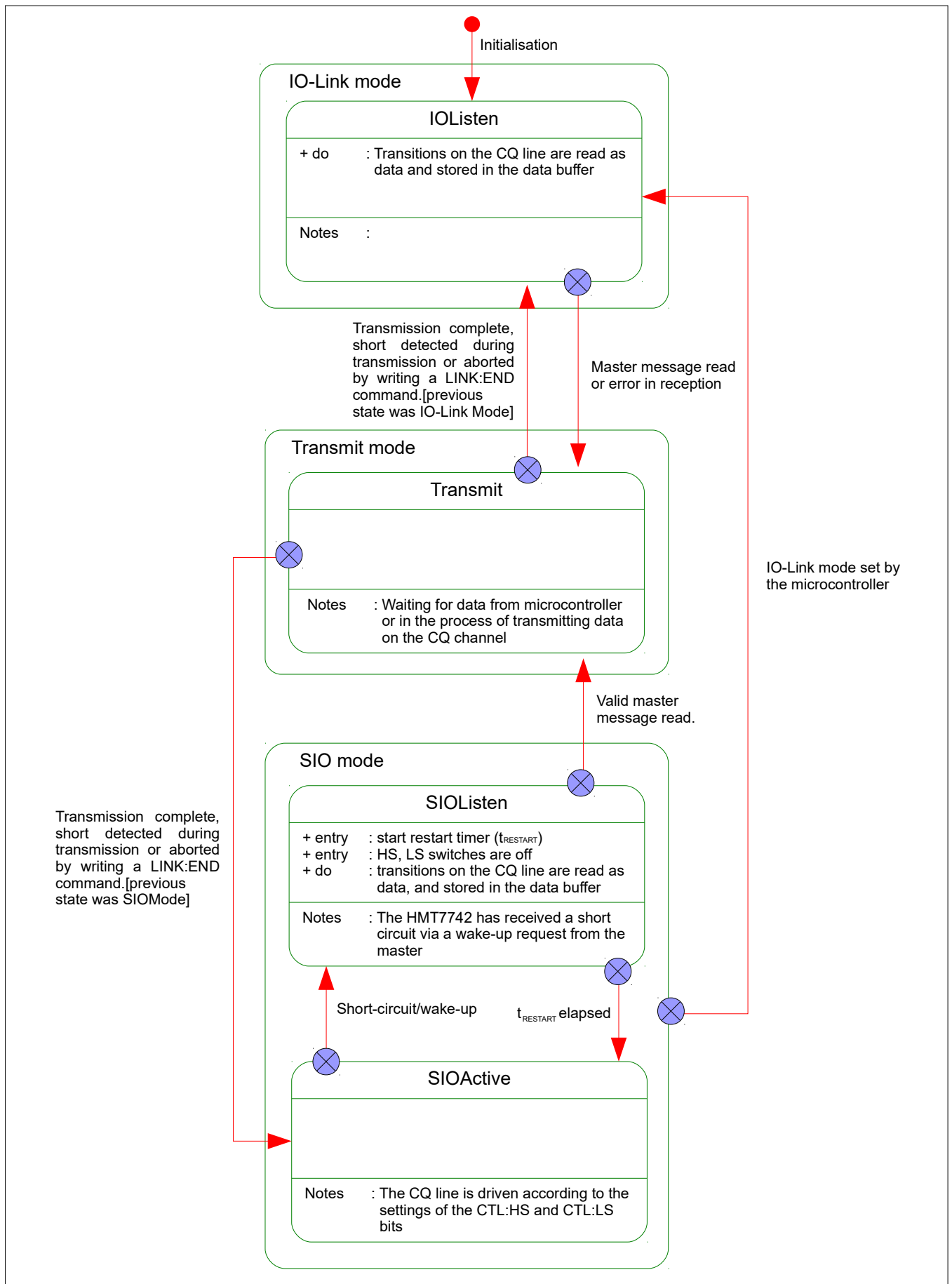
Fig. 6: IO-Link UART peripheral state machine
