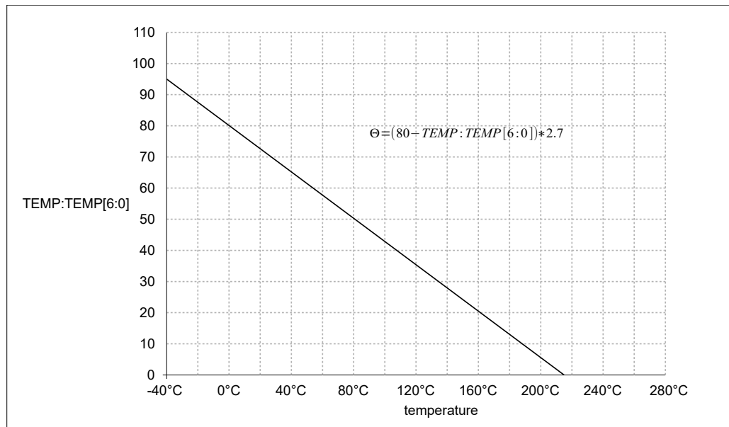
Fig. 9: HMT7742/3 temperature measurement
