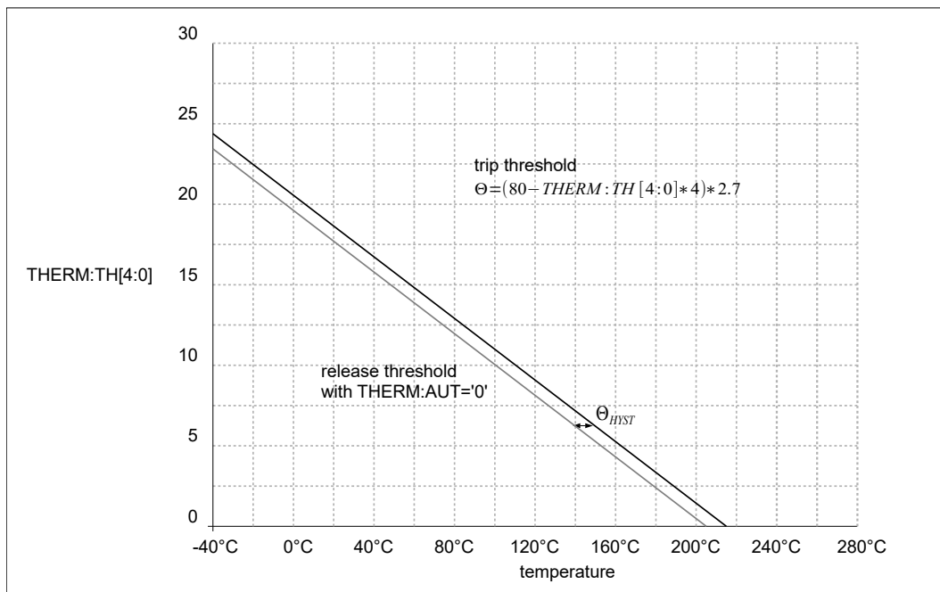
Fig. 10: HMT7742/3 temperature measurement
