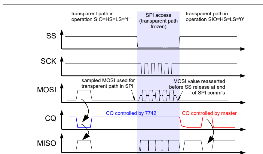
Fig. 8: Illustration of operation in transparent mode
