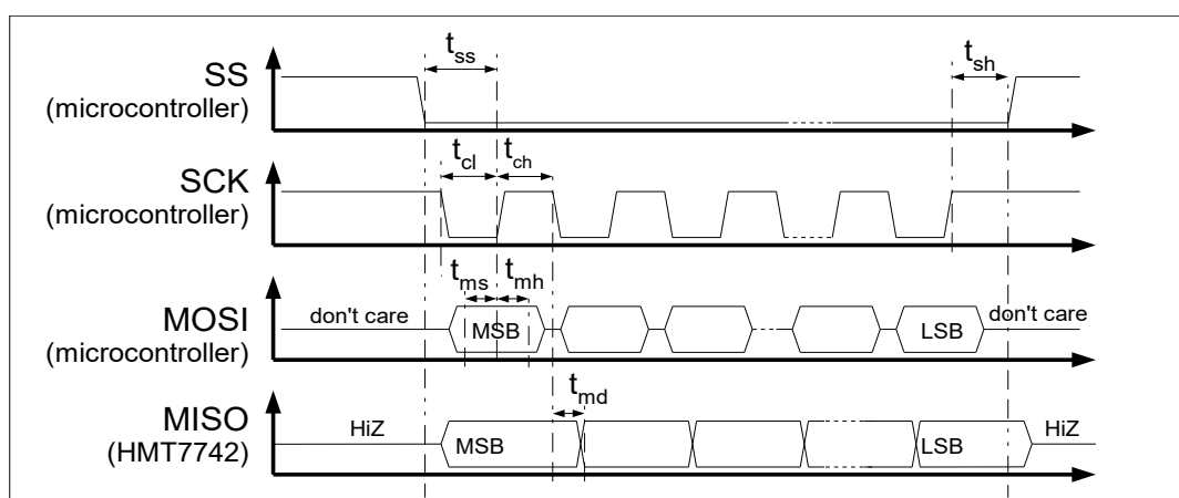
Fig. 4: Register programming
