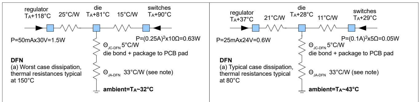
Fig. 14: Example thermal power dissipation estimation
