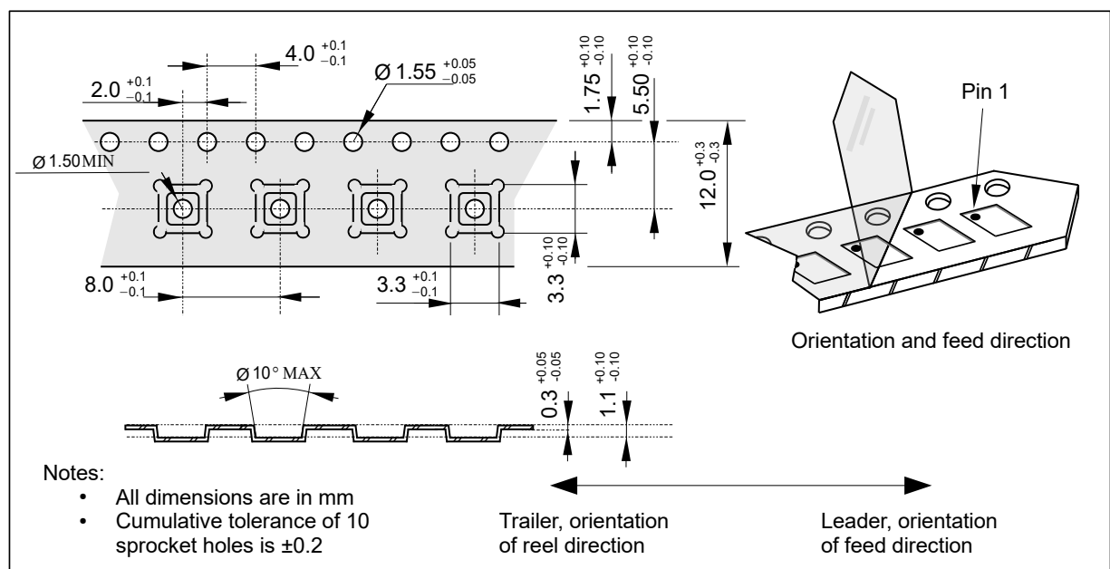
Fig. 17: Tape and Reel drawings
